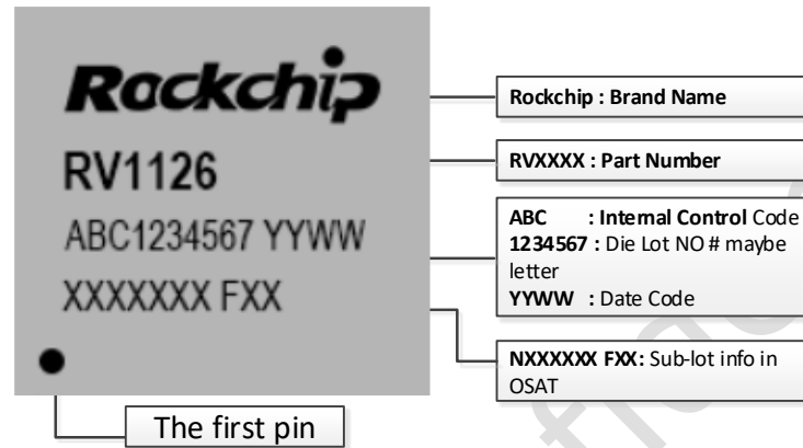
Fig.2-1 RV1126 Top marking
