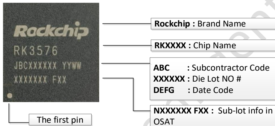
Fig.2-1 Package Definition
