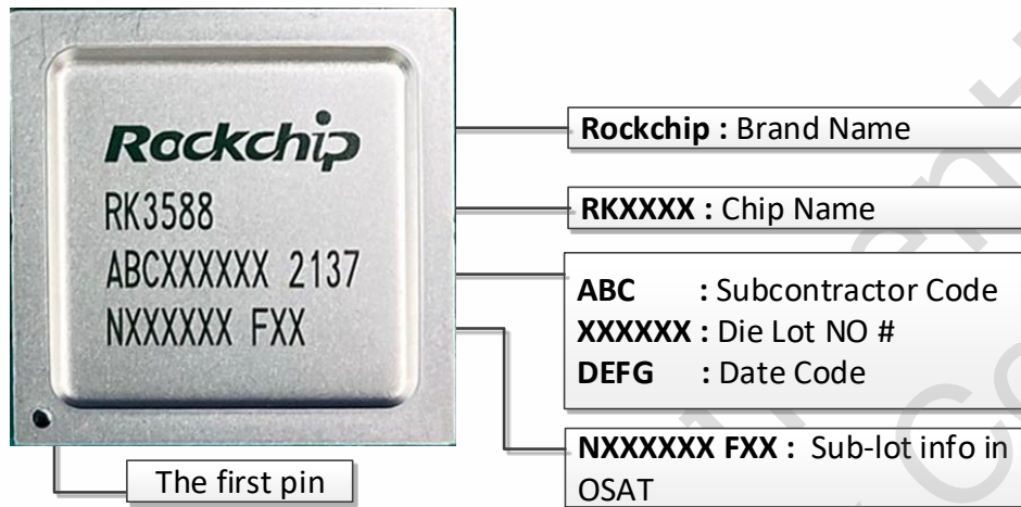
Fig.2-1 Package definition
